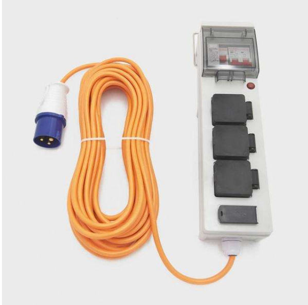
Typical electrical hook-up distribution unit for tents
